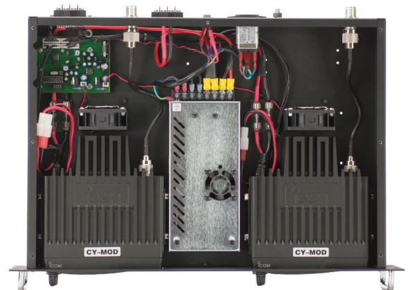
Radios, controller, and power supply, all in one box. Dual forced-air fans keep the unit cool. 19" Rack mountable. Battery backup capable.
