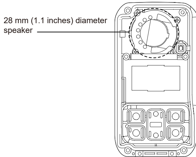
FRONT panel back view
