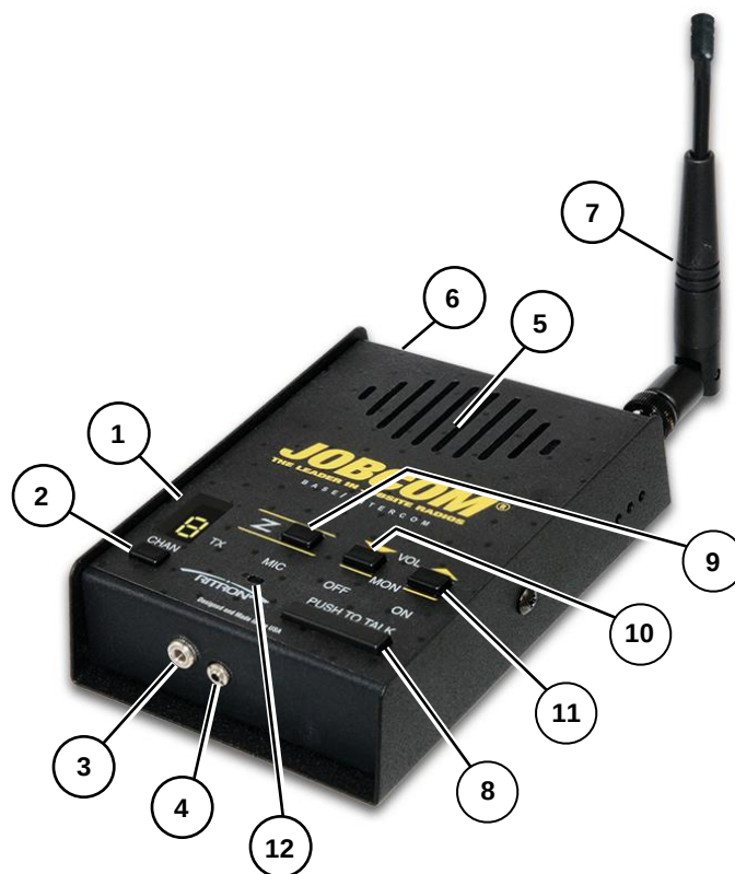
FIG-1: RADIO CONTROLS & CONNECTORS
